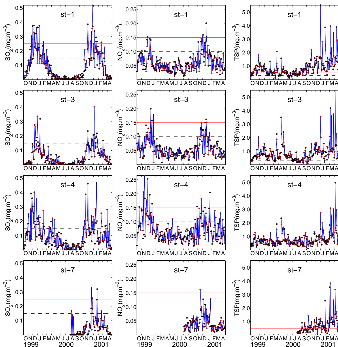
Figure 3. Daily mean \text{SO}_2 , \text{NO}_x , and TSP concentrations ( \text{mg m}^{-3} ) at St-1, St-3, St-4 and St-7. Horizontal dashed line is daily mean second-level standard, while horizontal solid line is daily mean third-level standard. Note that the daily mean TSP concentration is usually above the second-level standard.
