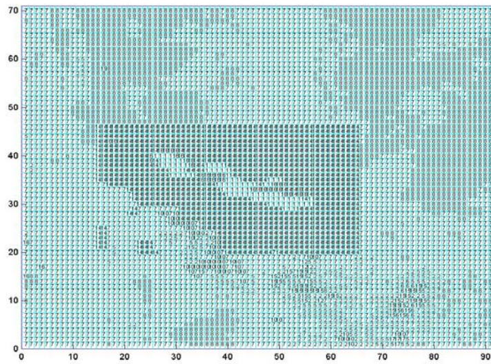
Figure 6. Surface condition for mountain-slope afforestation with the soil type-4. The soil type-4 is replaced by type-1 for experiment without mountain-slope afforestation.
