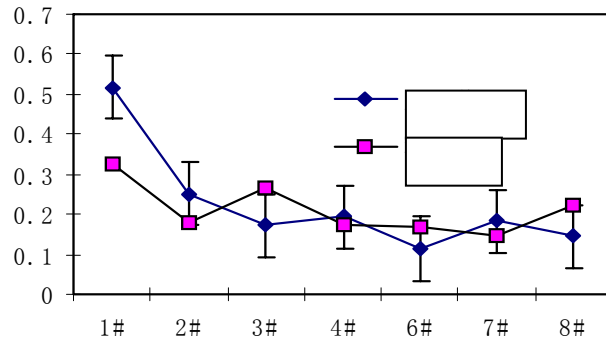
Figure 10. RAMS/HYPACT model verification. The horizontal axis represents station number, and the vertical axis represents observed and predicted SO 2 concentration (unit: mg/m 3 ).
